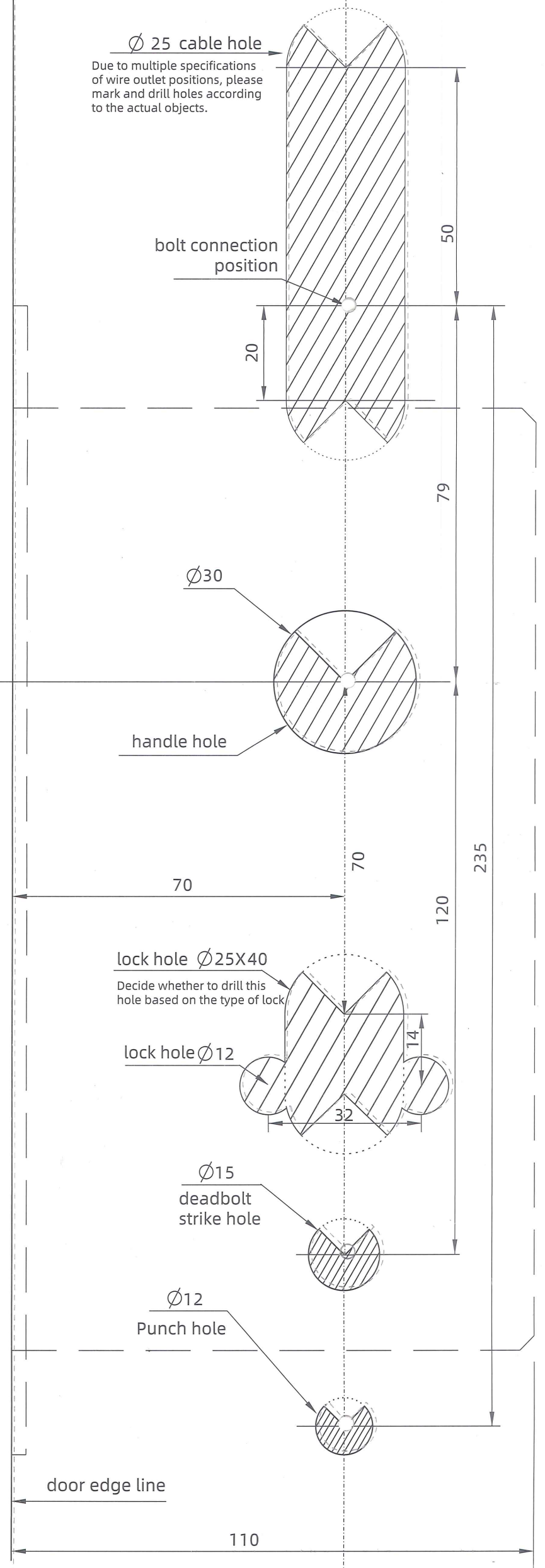
Panel hole dimensions
